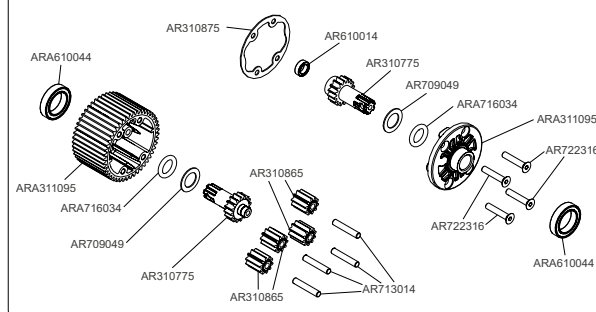
REAR DIFF EXPLODED VIEW
