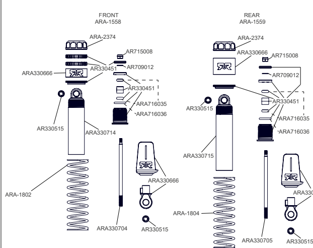
SHOCK ABSORBER EXPLODED VIEW
