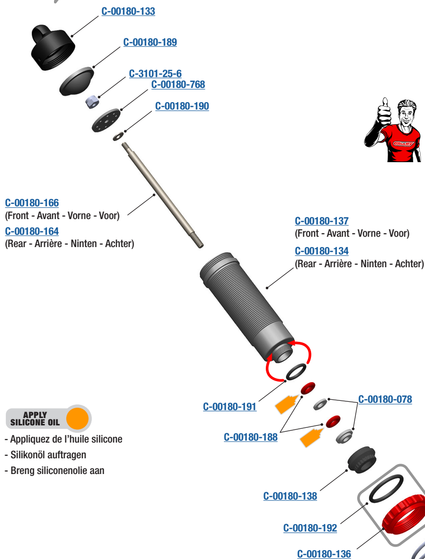
C-00180-768 Shock Piston (8pcs) Shock Piston - 6 Holes 1.4 Shock Piston - 8 Holes 1.2 (Factory installed)
